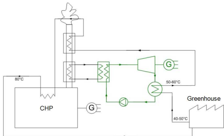
Figure 7 : ORC integrated within a CHP installation
