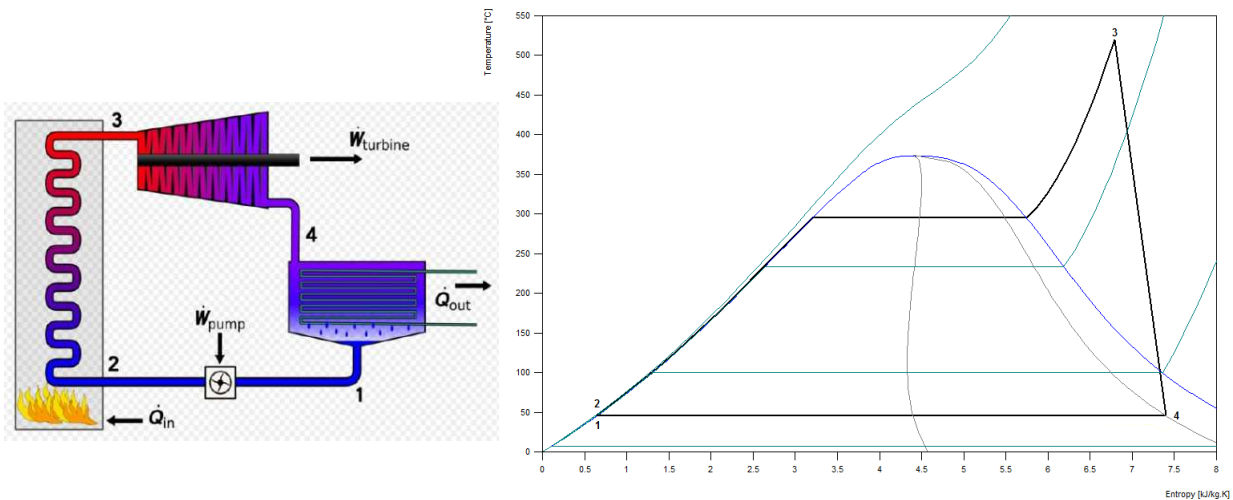
Figure 2 : T-s diagram of simplified steam cycle
