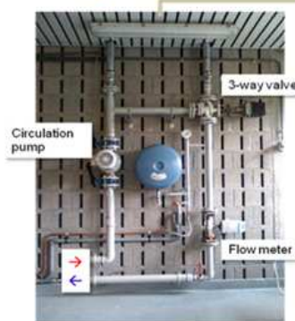
Figure 19 : Heat source, cooling loop, process control and monitoring, 11 kW e ORC
