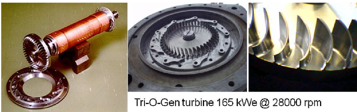
Figure 9 : Turbine used by Tri-O-Gen (source : Tri-O-Gen)
