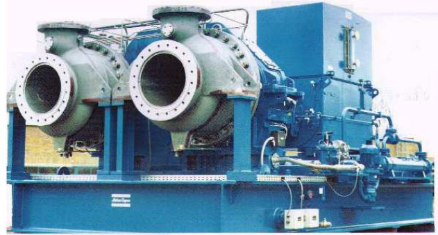
Figure 17 : 2-stage gas expansion turbine (Atlas Copco)
