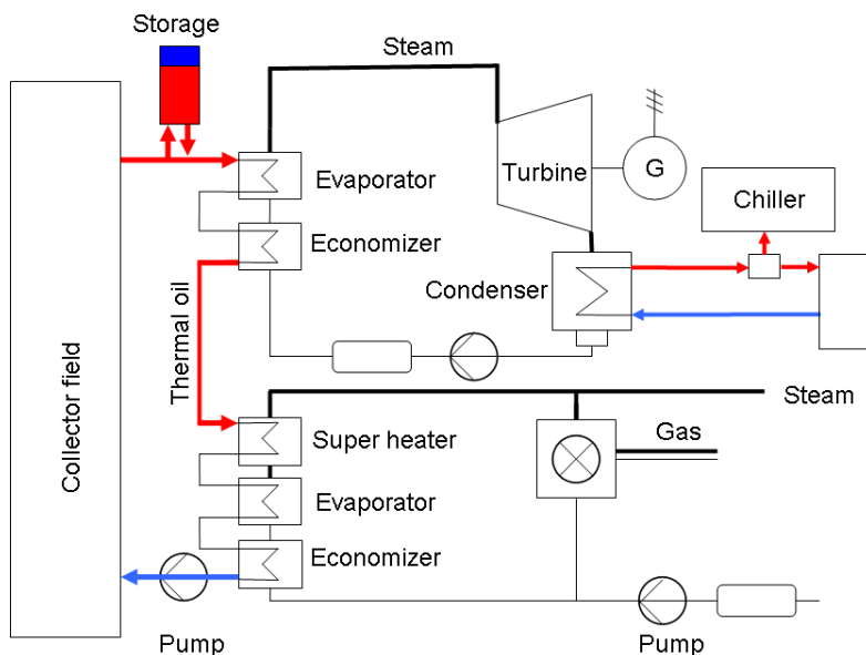
Figure 1: Possible cycle layout for solar polygeneration.
