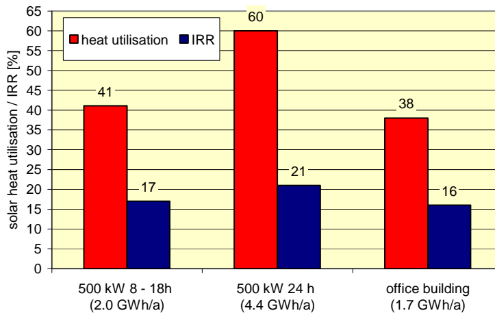
Figure 6: solar heat utilisation and internal rate of return for different cooling load profiles a) 500 kW during working hours 8-18h b) 500 kW 24h constant c) variable load for an office building (yearly demand in brackets)
