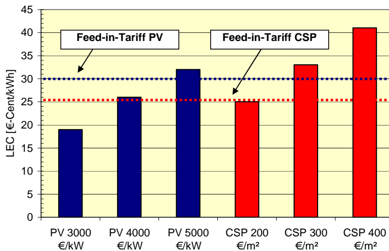
Figure 3: Levelised cost of electricity (LEC) for different solar field costs for photovoltaic power (PV) and concentrated solar thermal power (CSP) for grid-connected power systems
