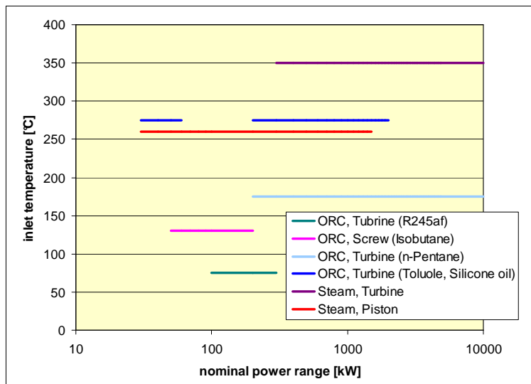
Figure 2: Overview on typical inlet temperatures and power ranges for various heat engines
