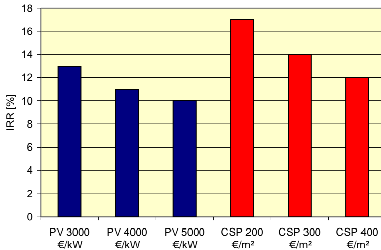
Figure 4: Internal rate of return (IRR) for equity invested in photovoltaic power (PV) and concentrated solar thermal power (CSP) in off-grid systems for different solar field costs
