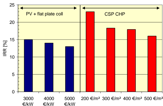
Figure 5: Internal rate of return (IRR) for equity invested in PV/Flat-plate solarthermal systems and concentrated solar thermal power (CSP) utilizing combined heat and power (CHP) for different solar field costs
