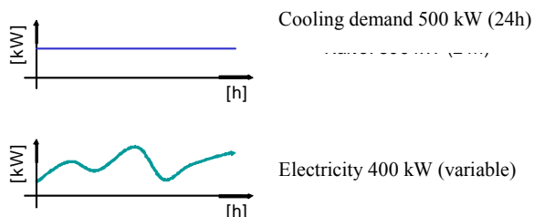
Figure 7: Demand profiles for combined cooling and power (CCP) in an off-grid industrial plant
